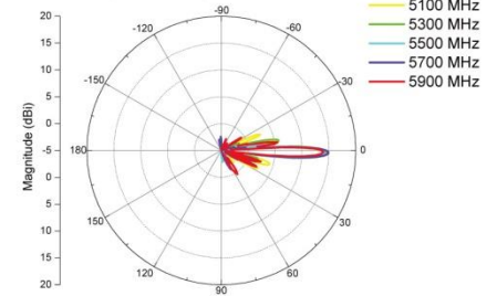
V-plane Co-polarization Pattern
