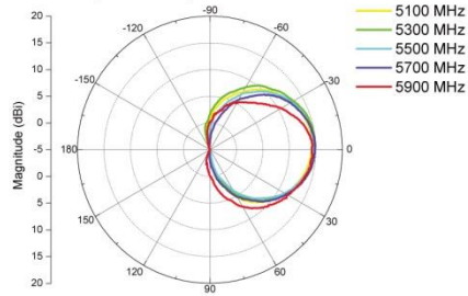
H-plane Co-polarization Pattern
