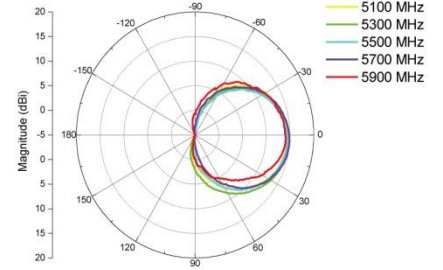
H-plane Co-polarization Pattern
